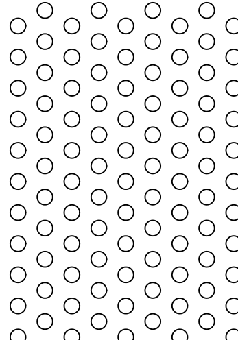
Perforering \varnothing 3 mm. Triangel delning 6 mm. Fri area 23%.
